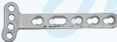
Distal Radius Volar Extra Articular LCP - 2.4mm (Left) Head With 4 Hole Mat:- S.S. / Titanium Cat No.: L.268.03.05 / T.275.03-05 Size:- 3,5 Hole
