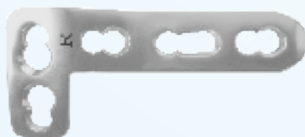
L Butteress Plate Locking Left/Right Mat:- S.S./ Titanium Cat No.: L210/211.03-10 / T224/225.03-10 Size:- 3 hole to 10 hole
