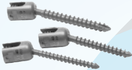
Polyaxial Screw Mat.: Titanium Cat No. SPI-PS45/55/65.25-50 Dia :- 4.5/5.5/6.5 MM Length : 25-50 MM
